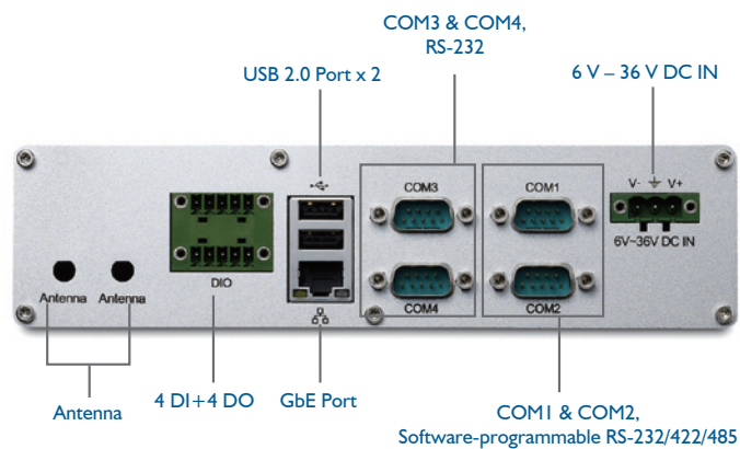
MXE-1300 Series Back Panel
